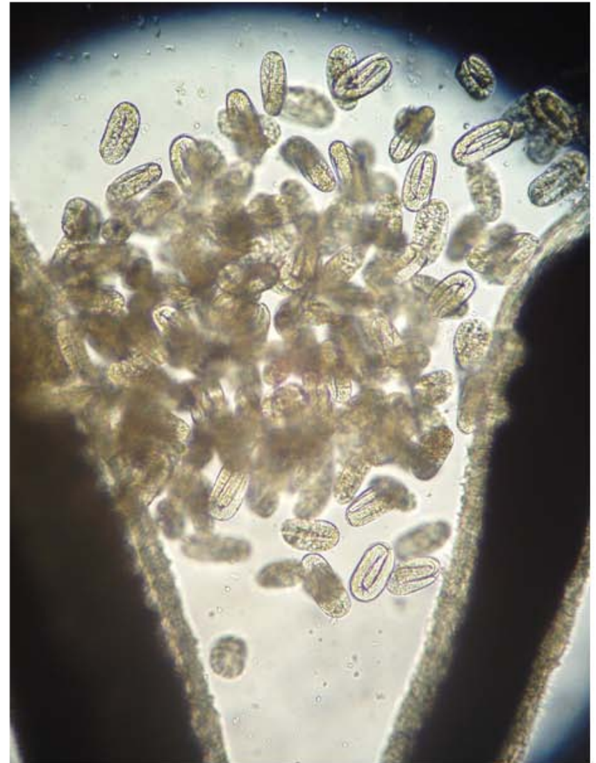
Lungworm; Rhabdias ranae (ex: Rana palustris ). Note larvated eggs.
